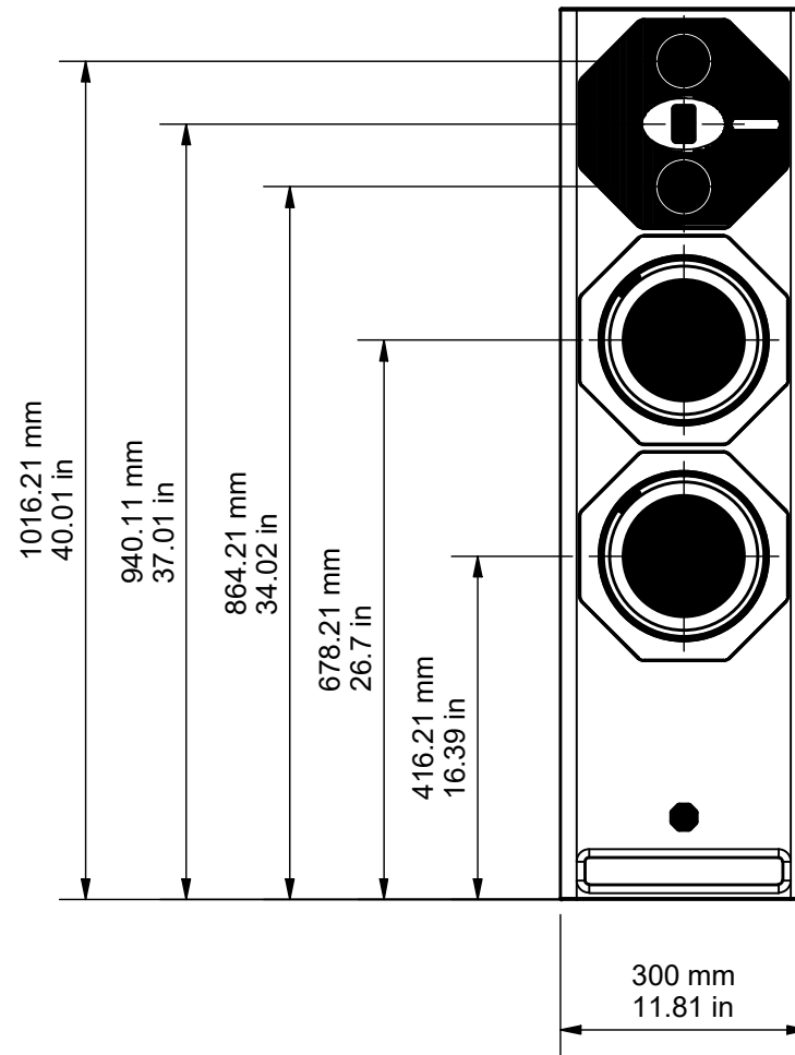
FRONT WITHOUT PLINTH (GRILLES OFF)
