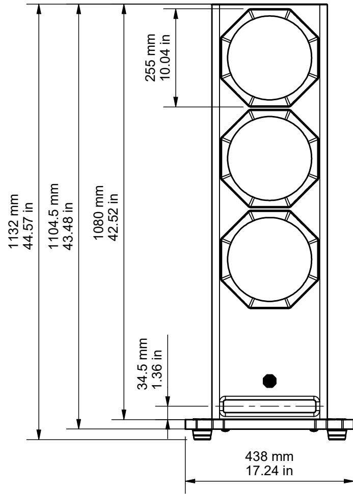
FRONT WITH PLINTH (GRILLES ON)
