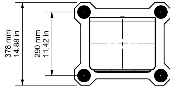
TOP WITH PLINTH
